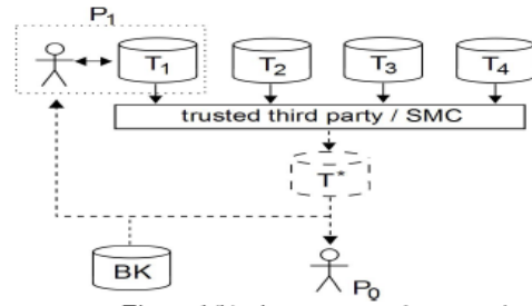
Figure 1(b). Aggregate-and-anonymize
