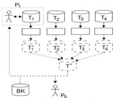
Figure 1(a). Anonymize-and-aggregate
