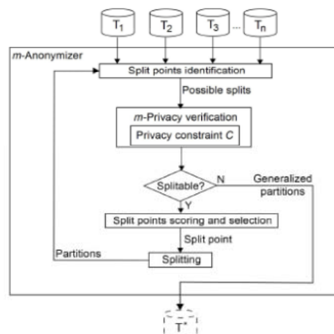
Figure 3. m -Anonymizer
